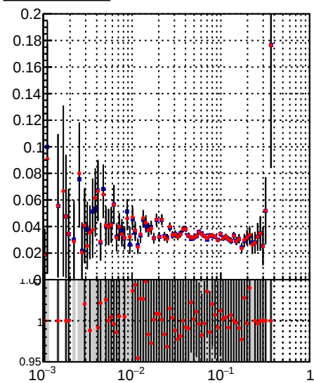
Fake rate vs \mu DQM_TT_mkFit-DQM_init_orig DQM_TT_mkFit-DQM_init_mod
