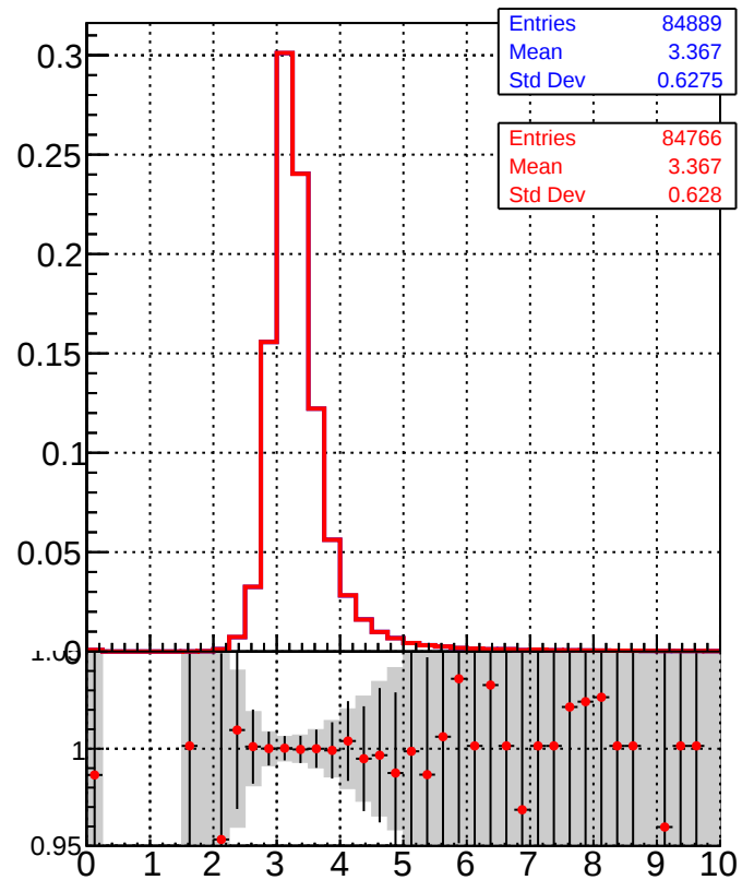
Legend: DQM_TT_mkFit-DQM_init_orig (gray histogram) DQM_TT_mkFit-DQM_init_mod (red line with points)
