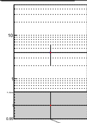
N of associated (recoToSim) tracks vs. s
