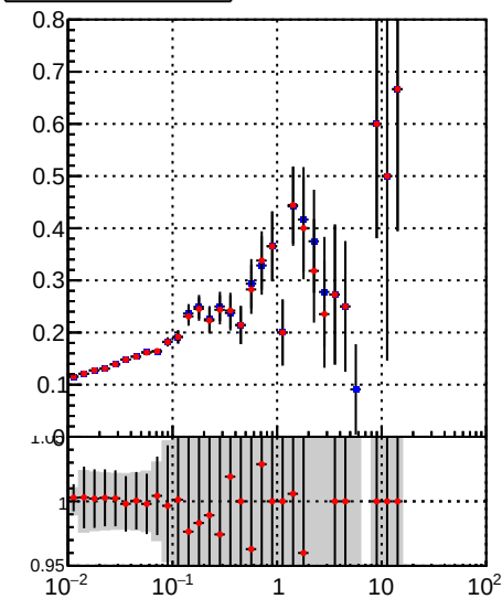
—•— DQM_TT_mkFit-DQM_init_orig —•— DQM_TT_mkFit-DQM_init_mod
