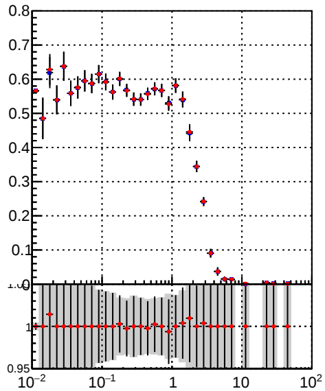
Efficiency vs. vertpos — DQM_TT_mkFit-DQM_init_orig — DQM_TT_mkFit-DQM_init_mod
