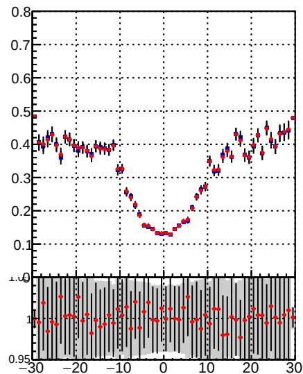
—●— DQM_TT_mkFit-DQM_init_orig —●— DQM_TT_mkFit-DQM_init_mod
