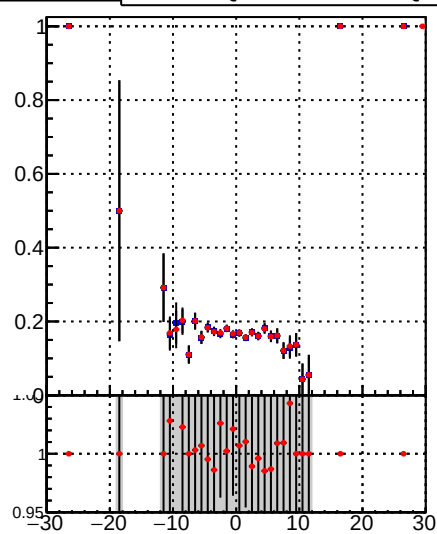
—•— DQM_TT_mkFit-DQM_init_orig —•— DQM_TT_mkFit-DQM_init_mod
