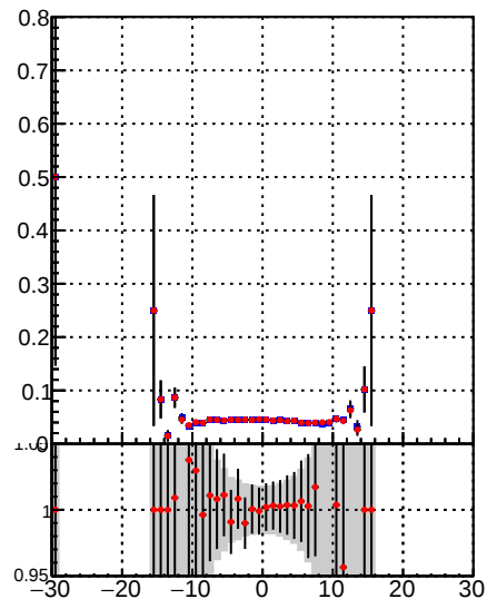
—●— DQM_TT_mkFit-DQM_init_orig —●— DQM_TT_mkFit-DQM_init_mod
