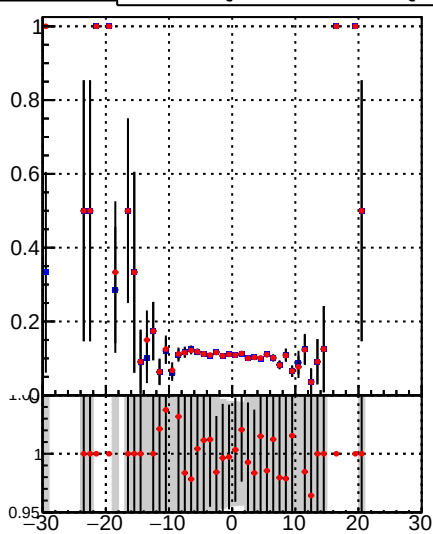
—■— DQM_TT_mkFit-DQM_init_orig —●— DQM_TT_mkFit-DQM_init_mod
