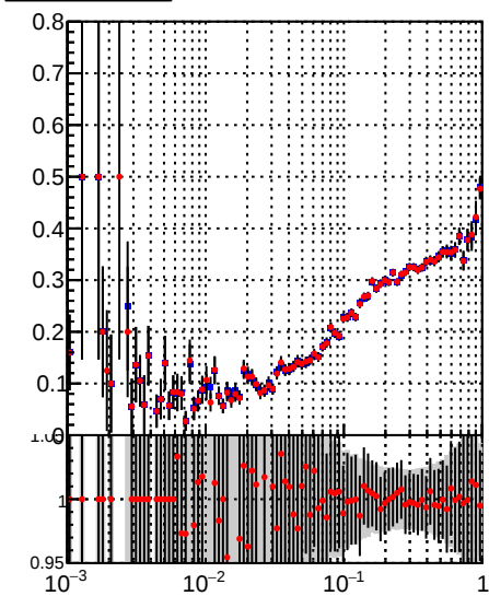
Fake rate vs \sqrt{s} Legend: DQM_TT_mkFit-DQM_init_orig (blue squares) DQM_TT_mkFit-DQM_init_mod (red circles)
