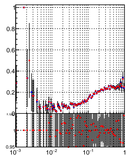
—●— DQM_TT_mkFit-DQM_init_orig —●— DQM_TT_mkFit-DQM_init_mod
