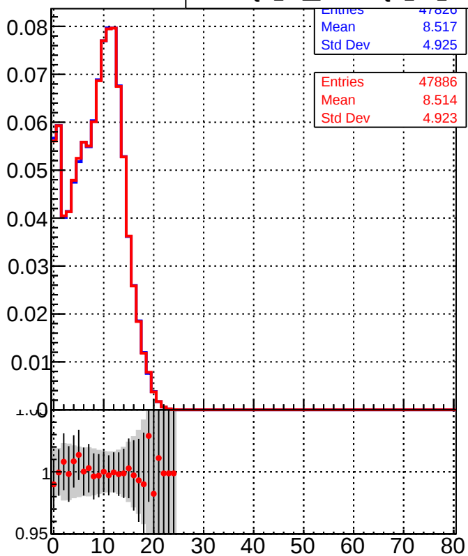
Legend for bottom row plots: DQM_TT_mkFit-DQM_init_orig (blue line with markers) DQM_TT_mkFit-DQM_init_mod (red line with markers)
