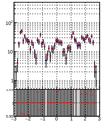
N of reco track vs \eta Legend: —•— DQM_TT_mkFit-DQM_init_orig —•— DQM_TT_mkFit-DQM_init_mod
