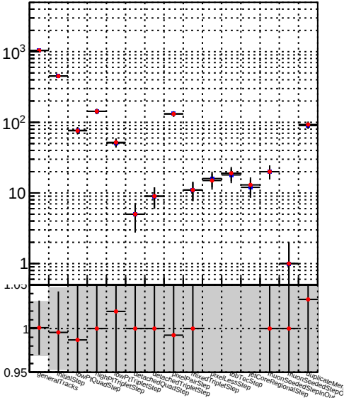
Number —●— DQM_TT__mkFit-DQM_init_mod
