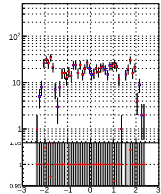
—•— DQM_TT_mkFit-DQM_init_orig —•— DQM_TT_mkFit-DQM_init_mod
