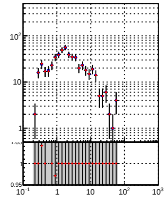
—•— DQM_TT_mkFit-DQM_init_orig —•— DQM_TT_mkFit-DQM_init_mod
