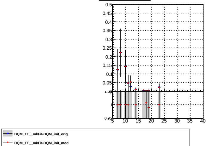
fake+duplicates vs pixel layers
