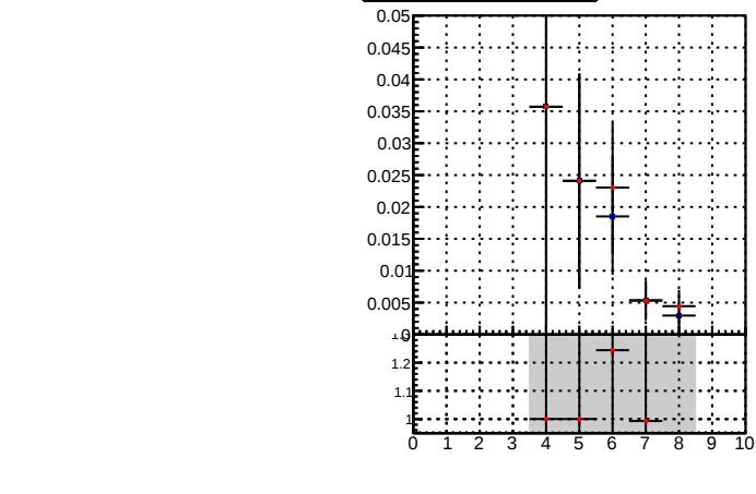
fake+duplicates vs 3D layers
