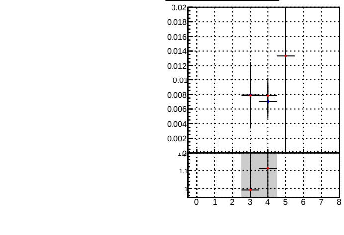
fake+duplicates vs 3D layers
