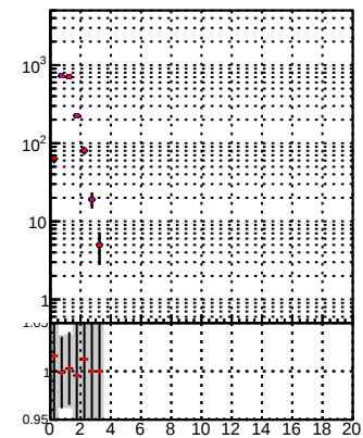
N of reco track vs. \chi^2 for DQM TT mkFit-DQM_init_orig and DQM TT mkFit-DQM_init_mod
