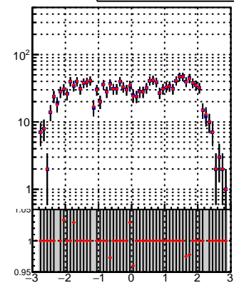
N of reco track vs \eta vs \phi —•— DQM TT mkFit-DQM_init_orig —•— DQM TT mkFit-DQM_init_mod
