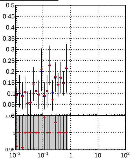
DQM_TT_mkFit-DQM_init_orig Fake rate vs \nu
