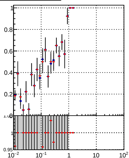
Pileup rate vs \nu
