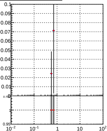
DQM_TT_mkFit-DQM_init_mod Duplicates Rate vs \nu
