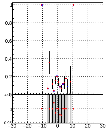
Fake rate vs d —●— DQM_TT_mkFit-DQM_init_orig —●— DQM_TT_mkFit-DQM_init_mod
