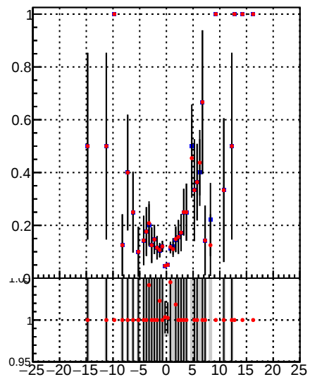
Fake rate vs d — \text{DQM\_TT\_mkFit-DQM\_init\_orig} — \text{DQM\_TT\_mkFit-DQM\_init\_mod}
