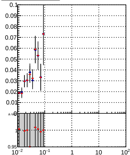
—•— DQM_TT_mkFit-DQM_init_orig —•— DQM_TT_mkFit-DQM_init_mod
