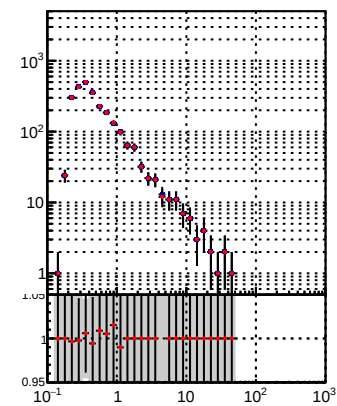
—•— DQM_TT_mkFit-DQM_init_orig —•— DQM_TT_mkFit-DQM_init_mod
