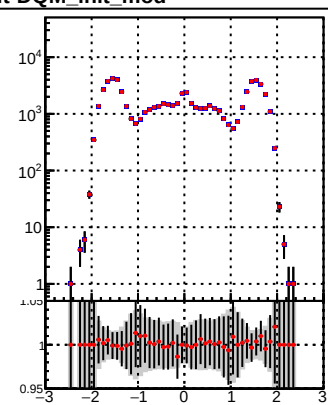
—•— DQM_TT_mkFit-DQM_init_orig —•— DQM_TT_mkFit-DQM_init_mod
