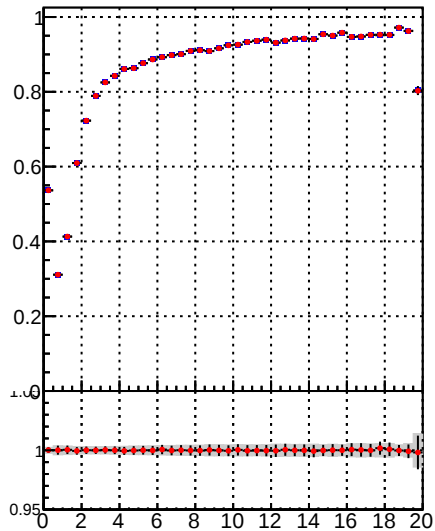
Fake rate vs. —•— DQM_TT_mkFit-DQM_init_orig —•— DQM_TT_mkFit-DQM_init_mod
