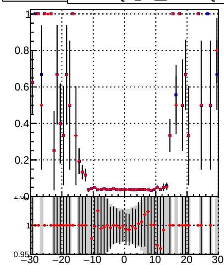
—●— DQM_TT_mkFit-DQM_init_orig —●— DQM_TT_mkFit-DQM_init_mod
