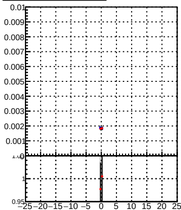
Duplicates Rate vs Dxyp(PV)
