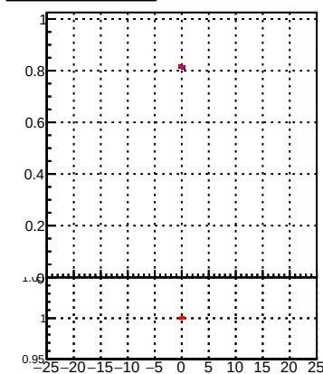
Pileup rate vs dxyp(PV)
