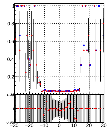
Fake rate vs d —●— DQM_TT_mkFit-DQM_init_orig —●— DQM_TT_mkFit-DQM_init_mod
