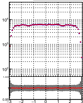
—●— DQM_TT_mkFit-DQM_init_orig —●— DQM_TT_mkFit-DQM_init_mod
