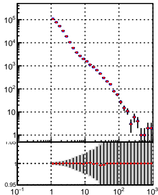
—●— DQM_TT_mkFit-DQM_init_orig —●— DQM_TT_mkFit-DQM_init_mod
