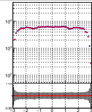
—●— DQM_TT_mkFit-DQM_init_orig —●— DQM_TT_mkFit-DQM_init_mod
