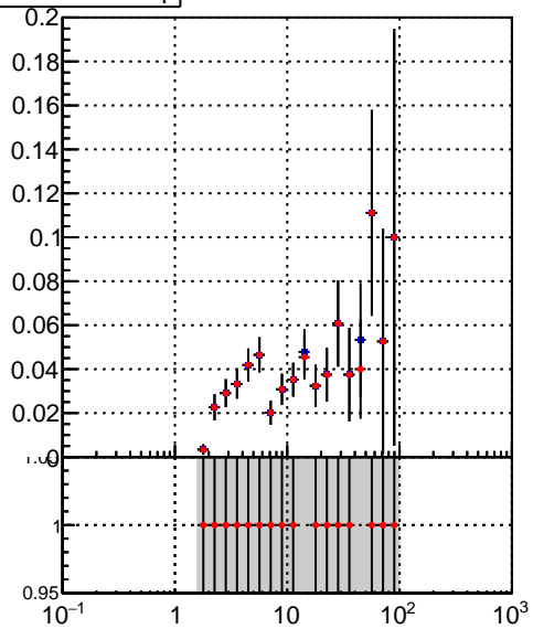
—■— DQM_TT_mkFit-DQM_init_orig —●— DQM_TT_mkFit-DQM_init_mod
