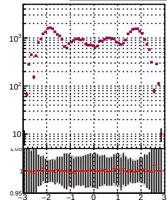
—•— DQM_TT_mkFit-DQM_init_orig —•— DQM_TT_mkFit-DQM_init_mod
