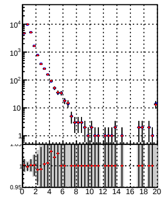
N of reco track vs. \chi^2 for DQM TT and mkFit-DQM_init_mod
