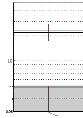
N of reco track vs. \chi^2 for different initialization methods
