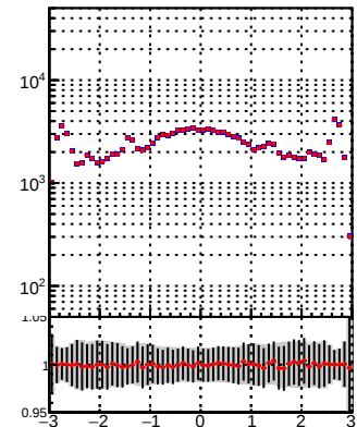
N of reco track vs \eta pT eta Legend: - Blue line with dots: DQM_TT_mkFit-DQM_init_orig - Red line with dots: DQM_TT_mkFit-DQM_init_mod
