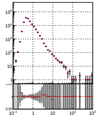
N of reco track vs \eta pT [GeV] ● DQM_TT_mkFit-DQM_init_orig ● DQM_TT_mkFit-DQM_init_mod
