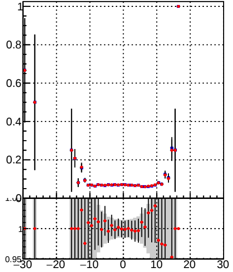
Efficiency vs. sim PV z Legend: DQM_TT_mkFit-DQM_init_orig (blue squares) DQM_TT_mkFit-DQM_init_mod (red crosses)
