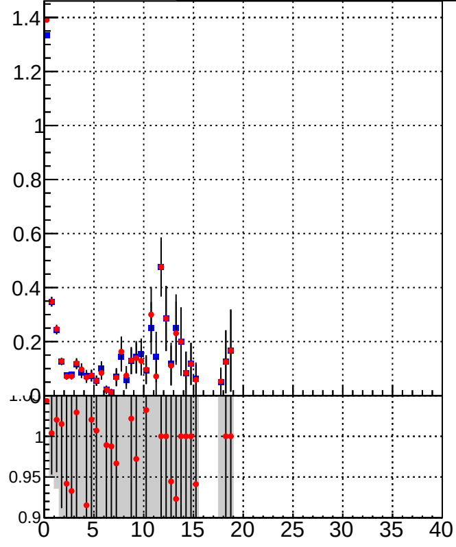
K_S^0 tracking fake rate vs p_T and \eta Legend: \blacksquare DQM_TT_mkFit-DQM_init_orig \bullet DQM_TT_mkFit-DQM_init_mod
