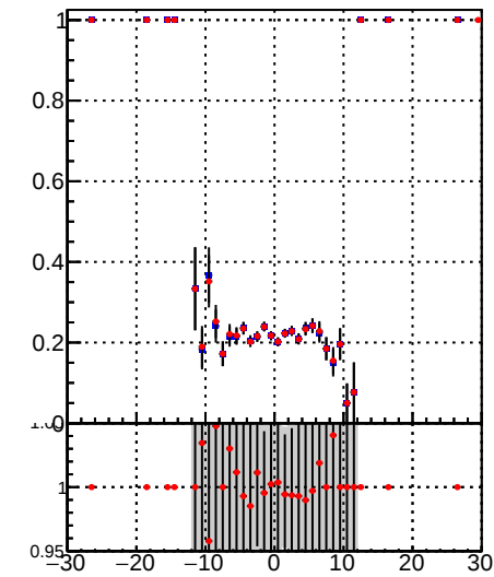
—■— DQM_TT_mkFit-DQM_init_orig —●— DQM_TT_mkFit-DQM_init_mod
