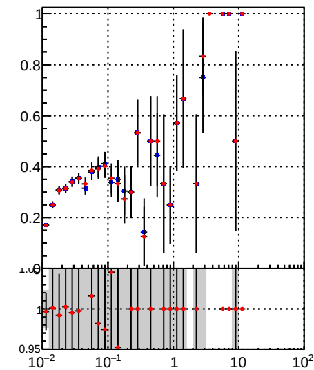
—■— DQM_TT_mkFit-DQM_init_orig —●— DQM_TT_mkFit-DQM_init_mod
