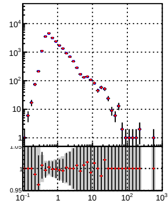
—●— DQM_TT_mkFit-DQM_init_orig —●— DQM_TT_mkFit-DQM_init_mod
