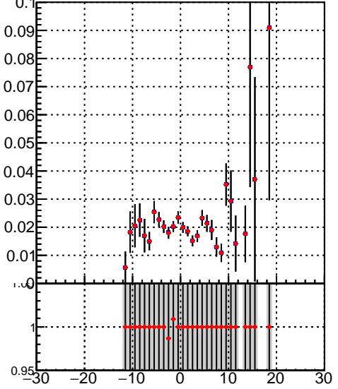
Efficiency vs vertpos — DQM_TT_mkFit-DQM_init_orig — DQM_TT_mkFit-DQM_init_mod
