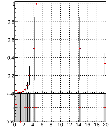
Fake rate vs. DQM_TT_mkFit-DQM_init_orig DQM_TT_mkFit-DQM_init_mod
