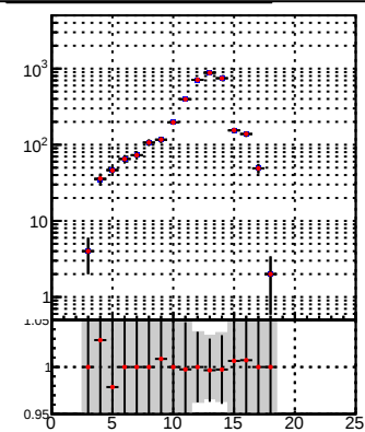
DQM_TT_mkFit-DQM_init_orig DQM_TT_mkFit-DQM_init_mod
