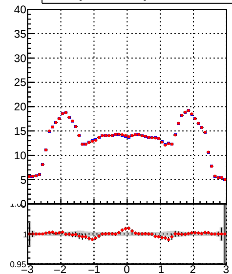
— DQM_TT_mkFit-DQM_init_orig — DQM_TT_mkFit-DQM_init_mod
