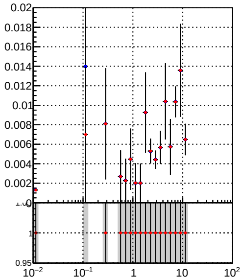
Efficiency vs vertpos Legend: DQM_TT_mkFit-DQM_init_orig DQM_TT_mkFit-DQM_init_modi3
