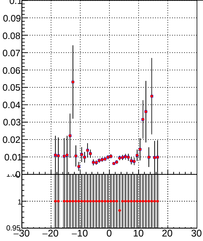
Efficiency vs Dz Legend: DQM_TT_mkFit-DQM_init_orig (Blue square) DQM_TT_mkFit-DQM_init_modi3 (Red circle)
