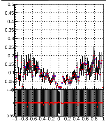
Efficiency vs Dxy(PV) Legend: DQM_TT_mkFit-DQM_init_orig (black line with error bars), DQM_TT_mkFit-DQM_init_modi3 (red line with error bars)
