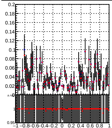
Efficiency vs Dxy(PV) Legend: DQM_TT_mkFit-DQM_init_orig DQM_TT_mkFit-DQM_init_modi3
