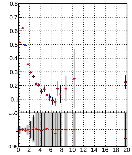
Fake rate vs. —●— DQM_TT_mkFit-DQM_init_orig —●— DQM_TT_mkFit-DQM_init_mod3
