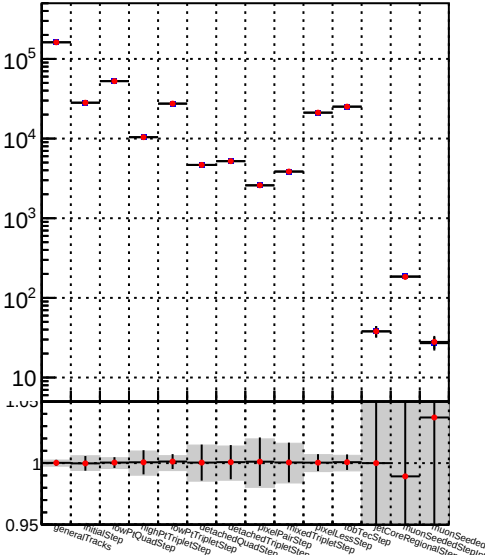
Number —●— DQM_TT_mkFit-DQM_init_modi3
