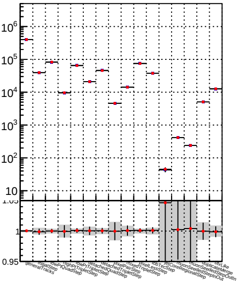
Number —●— DQM_TT_mkFit-DQM_init_modi3
